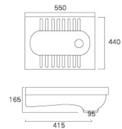
Squatting Pan LD1509Q Size(mm): 550×440×165 Drainage Outlet: Forward outlet, No integrated S-trap
