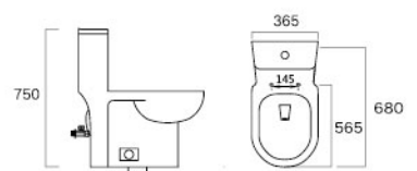
Siphonic One-piece Toilet LZ2202M/L Size(mm): 680×365×750 Roughing-in(mm): M 300/L 400 Water Consumption: 5.0L
