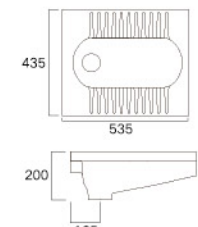
Squatting Pan LD1322 NEW! Size(mm): 535×435×200 Drainage Outlet: Backward outlet, No integrated S-trap
