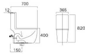
Siphonic One-piece Toilet LZ1225M/L Size(mm): 700×365×820 Roughing-in(mm): M 300/L 400 Water Consumption: 5.0L
