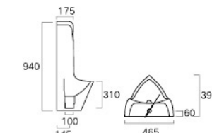
Pedestal Urinal LX1203 Size(mm): 465×390×940 Drainage Outlet: Vertical outlet Including hook accessories, Not including metal joint pipe, flashing valve, sensor
