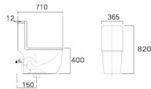
Siphonic One-piece Toilet LZ1226M/L Size(mm): 710×365×820 Roughing-in(mm): M 300/L 400 Water Consumption: 5.0L
