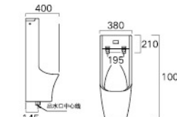
Pedestal Urinal LX1204 Size(mm): 380×400×1000 Drainage Outlet: Vertical outlet Including hook accessories, shower nozzle, sensor
