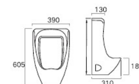
Wall Hung Urinal LX1304H Size(mm): 390×310×605 Drainage Outlet: Horizontal Outlet Including hook accessories, Not including metal joint pipe, flashing valve, sensor
