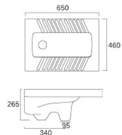
Squatting Pan LD1507Q Size(mm): 650×460×265 Drainage Outlet: Forward outlet, Integrated S-trap
