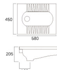
Squatting Pan LD1323 NEW! Size(mm): 580×450×205 Drainage Outlet: Backward outlet, No integrated S-trap
