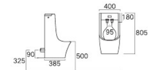
Wall Hung Urinal LX1306H Size(mm): 400×385×805 Drainage Outlet: Horizontal Outlet Including hook accessories, shower nozzle, sensor
