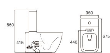
Washdown Two-piece Toilet LZ1603 P/S NEW! Size(mm): 675×360×860 Roughing-in(mm): Horizontal Outlet 180 / S Vertical Outlet 200 Water Consumption: 5.0L
