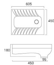
Squatting Pan LD1508Q Size(mm): 605×450×180 Drainage Outlet: Forward outlet, No integrated S-trap
