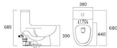
Siphonic One-piece Toilet LZ1230M/L Size(mm): 680×380×685 Roughing-in(mm): M 300/L 400 Water Consumption: 5.0L
