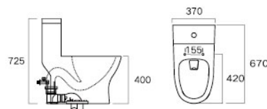
Siphonic One-piece Toilet LZ1224M/L Size(mm): 670×370×725 Roughing-in(mm): M 300/L 400 Water Consumption: 5.0L
