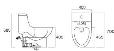
Siphonic One-piece Toilet LZ1228M/L Size(mm): 700×400×685 Roughing-in(mm): M 300/L 400 Water Consumption: 5.0L
