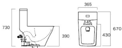
Siphonic One-piece Toilet LZ1223M/L Size(mm): 670×365×730 Roughing-in(mm): M 300/L 400 Water Consumption: 5.0L
