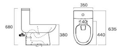
Washdown One-piece Toilet LZ2201M/L Size(mm): 635×350×680 Roughing-in(mm): M 300/L 400 Water Consumption: 5.0L
