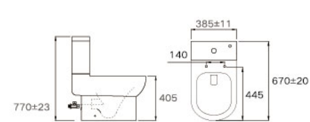
Washdown Two-piece Toilet LZ1602 P/S NEW! Size(mm): 670×385×770 Roughing-in(mm): Horizontal Outlet 180 / S Vertical Outlet 200 Water Consumption: 5.0L
