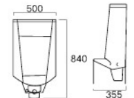
Wall Hung Urinal LX1305H Size(mm): 500×355×840 Drainage Outlet: Horizontal Outlet Including hook accessories, Not including sensor
