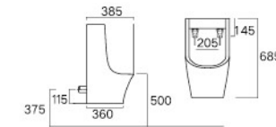
Wall Hung Urinal LX1307H Size(mm): 360×385×685 Drainage Outlet: Horizontal Outlet Including hook accessories, shower nozzle and L-Type metal joint pipe, Not including sensor
