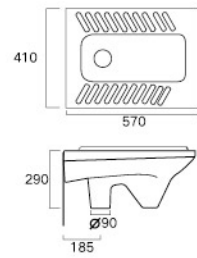
Squatting Pan LD1506Q Size(mm): 570×410×290 Drainage Outlet: Backward outlet, Integrated S-trap
