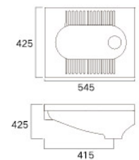
Squatting Pan LD1321 NEW! Size(mm): 545×425×205 Drainage Outlet: Forward outlet, No integrated S-trap
