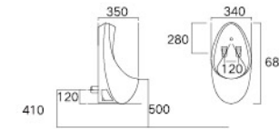
Wall Hung Urinal LX1308H Size(mm): 350×340×680 Drainage Outlet: Horizontal Outlet Including hook accessories, shower nozzle, Not including sensor
