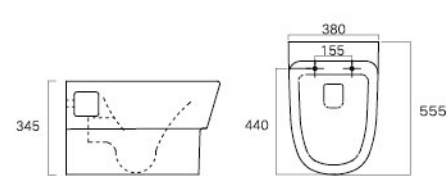
Wall Hung Toilet LZ1301 Size(mm): 555×380×345 Roughing-in(mm): Horizontal Outlet Water Consumption: 5.0L
